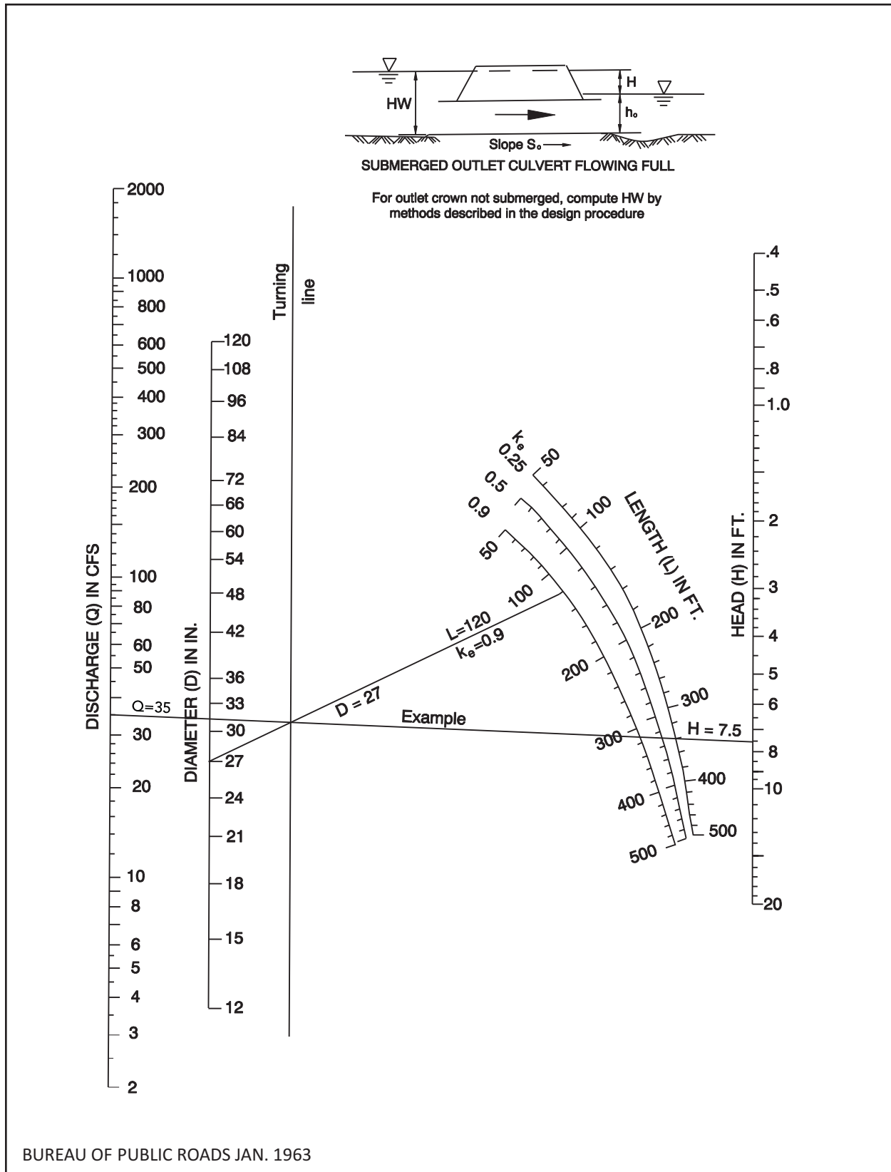
Figure 4-A-2 Head For Standard C. M. Pipe Culverts Flowing Full n = 0.024
