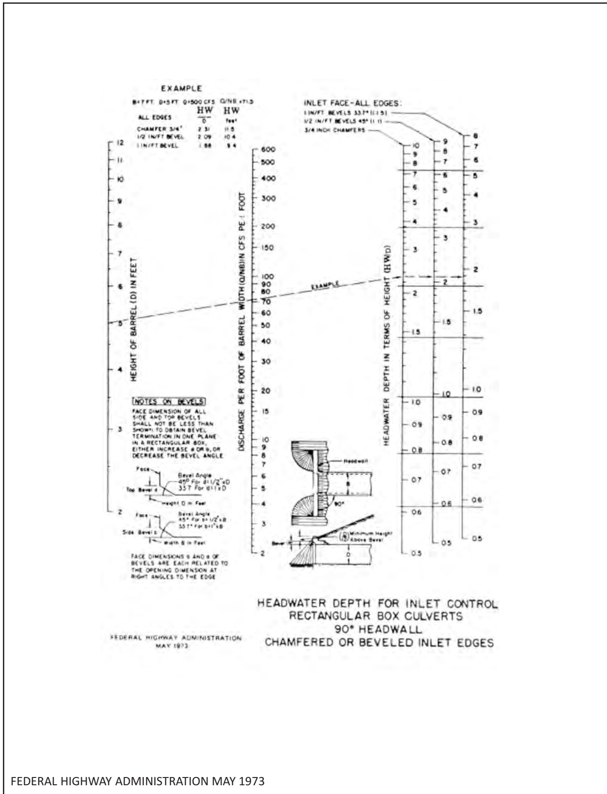
Figure 4-C-2 Headwater Depth For Inlet Control Rectangular Box Culverts 90° Headwall Chamfered Or Beveled Inlet Edges
