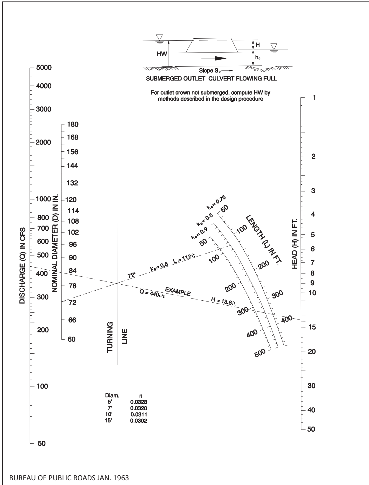
Figure 4-A-4 Head For Structural Plate Corr. Metal Pipe Culverts Flowing Full n = 0.0328 to 0.0302
