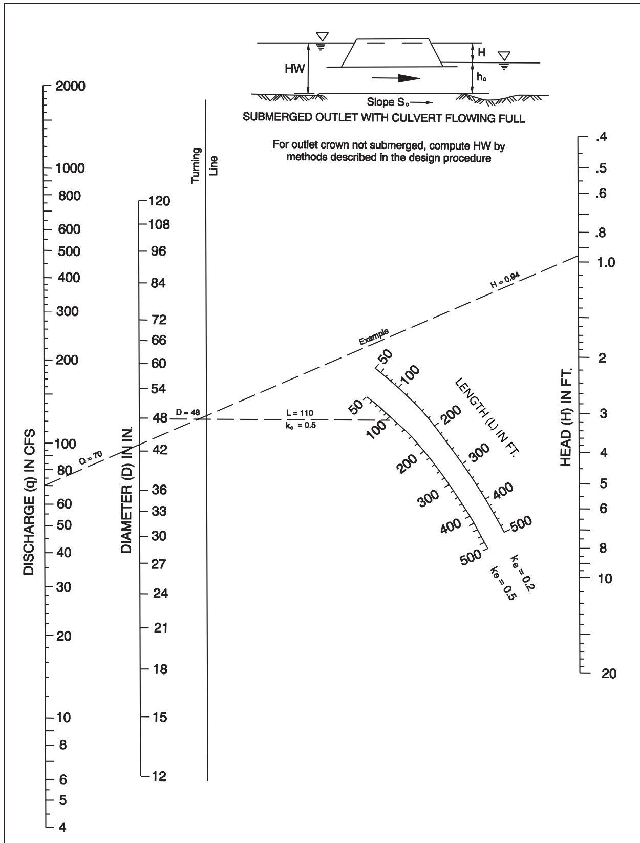
Figure 4-3 Head for Concrete Pipe Culverts Flowing Full (n = 0.012)
