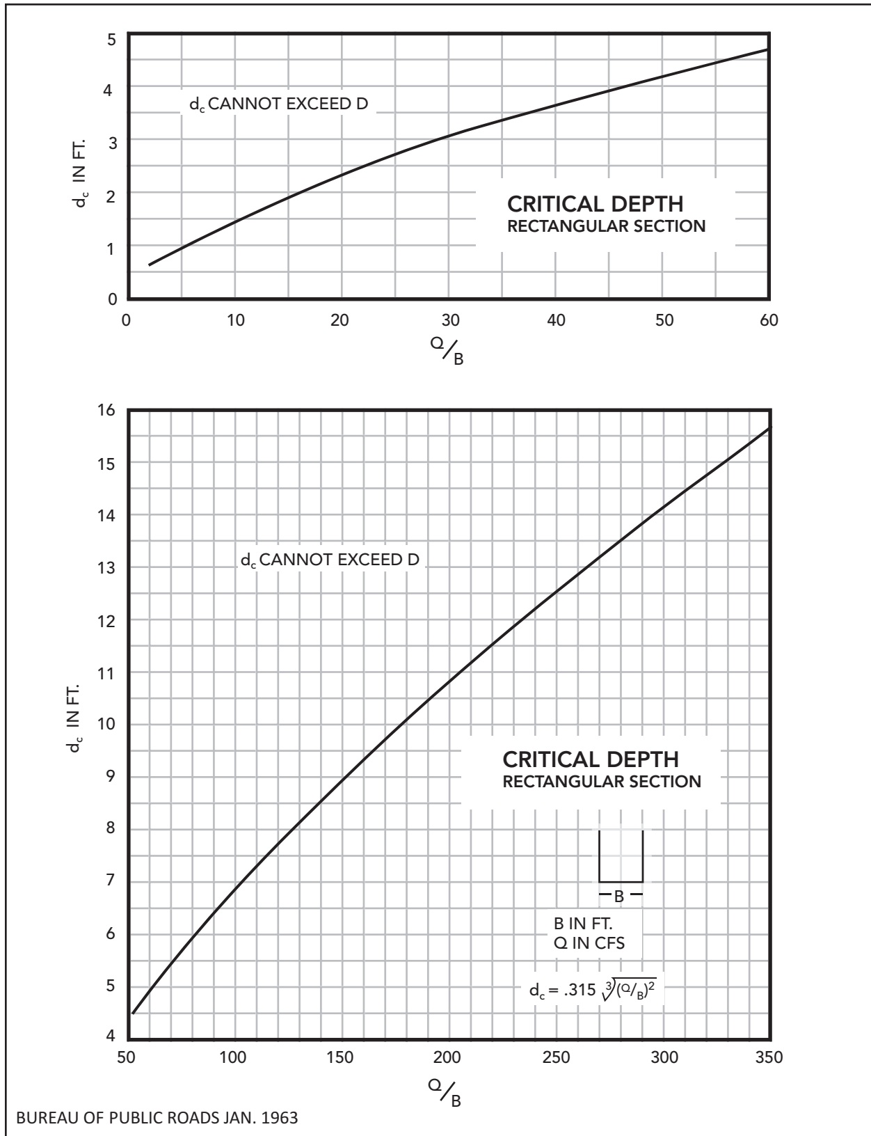
Figure 4-B-2 Critical Depth Rectangular Section
