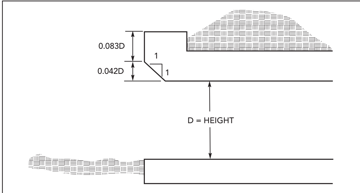
Figure 4-6 Beveled Edged Inlet
