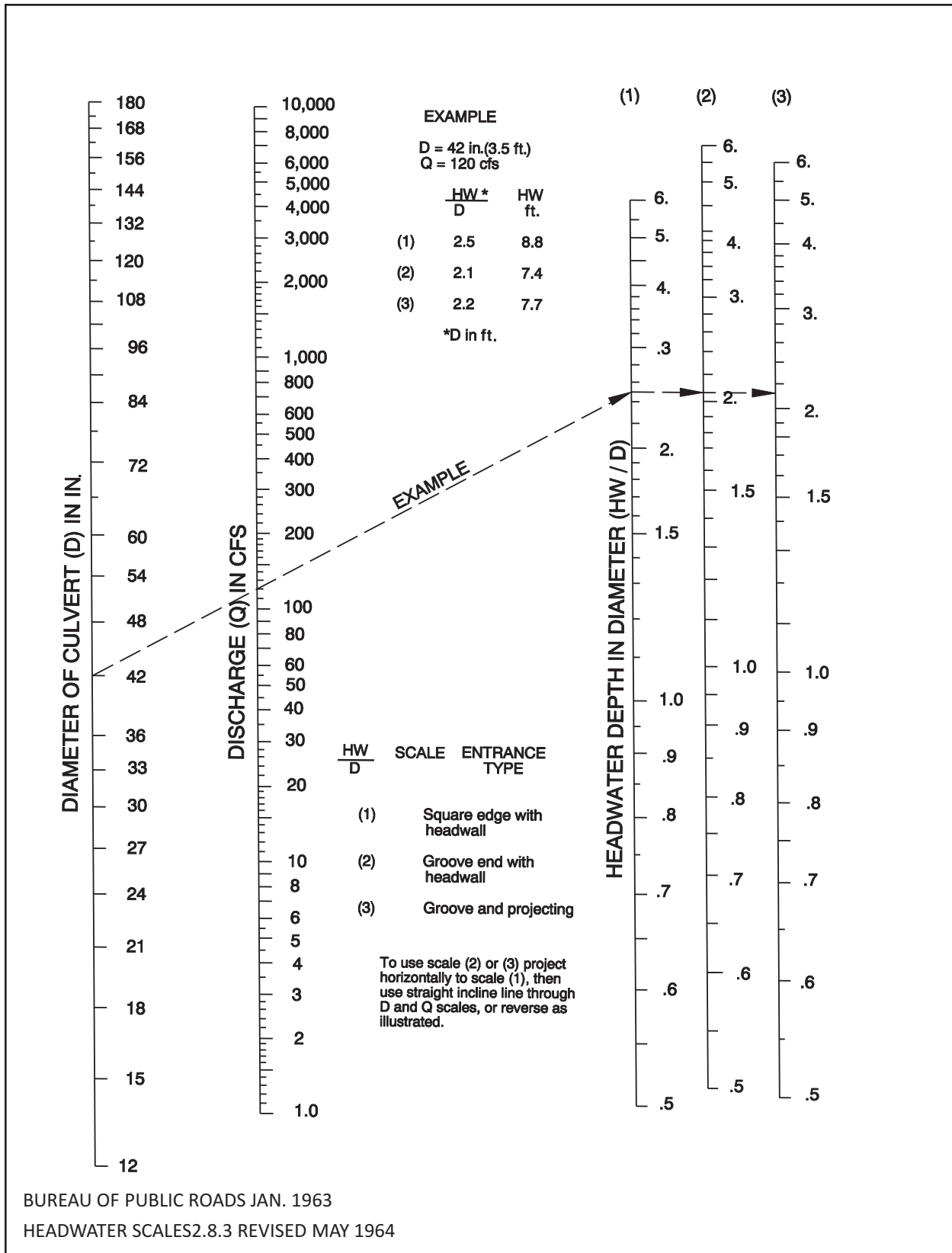
Figure 4-A-6 Headwater Depth For Concrete Pipe Culverts With Inlet Control
