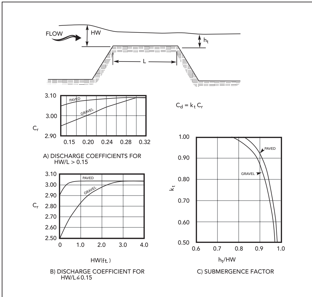
Figure 4-4 Discharge Coefficients for Roadway Overtopping
