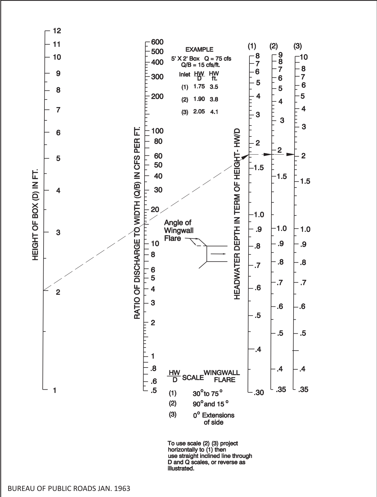
Figure 4-A-7 Headwater Depth For Box Culverts With Inlet Control
