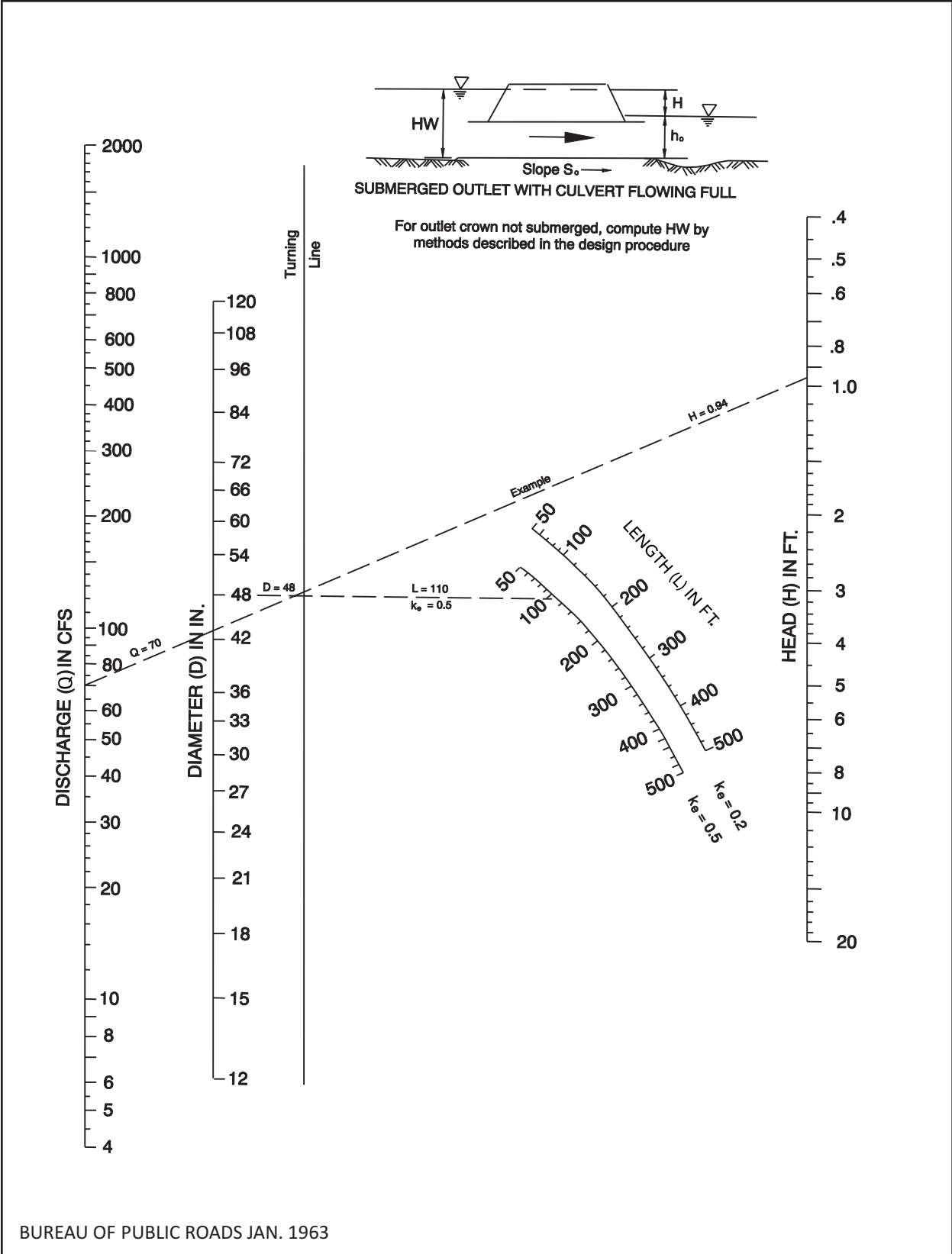
Figure 4-A-1 Head For Concrete Pipe Culverts Flowing Full n = 0.012
