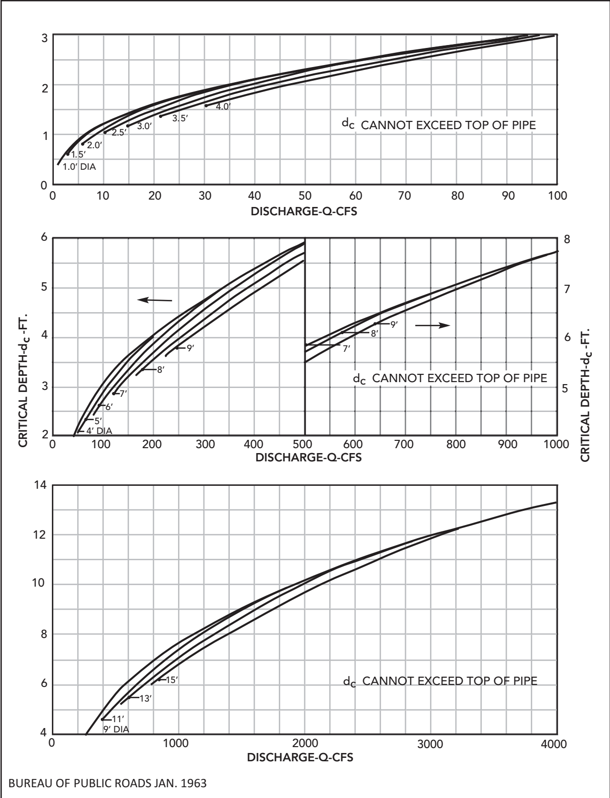
Figure 4-B-1 Critical Depth Circular Pipe
