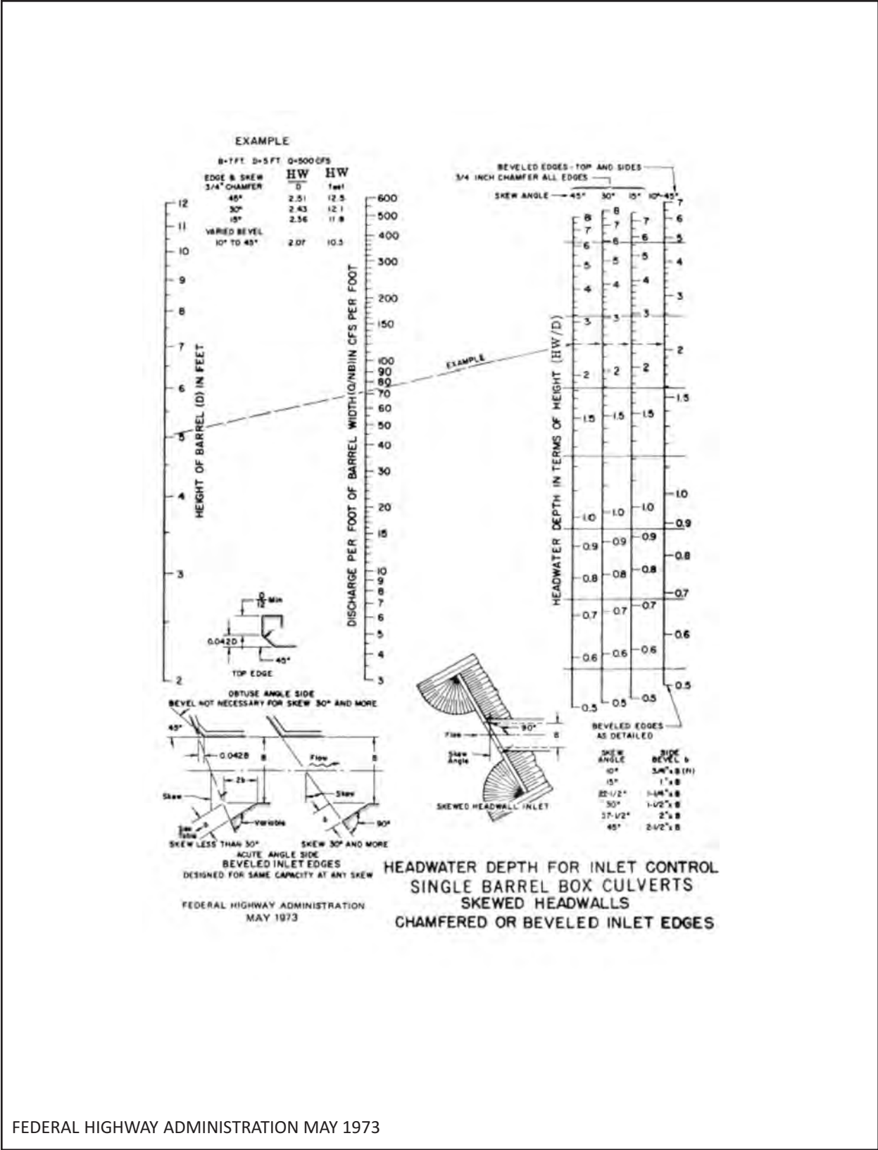
Figure 4-C-3 Headwater Depth For Inlet Control Single Barrel Box Culverts Skewed Headwalls Chamfered Or Beveled Inlet Edges
