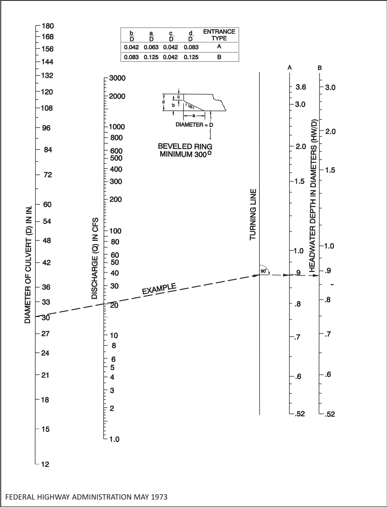
Figure 4-C-1 Headwater Depth For Circular Pipe Culverts With Beveled Ring Inlet Control
