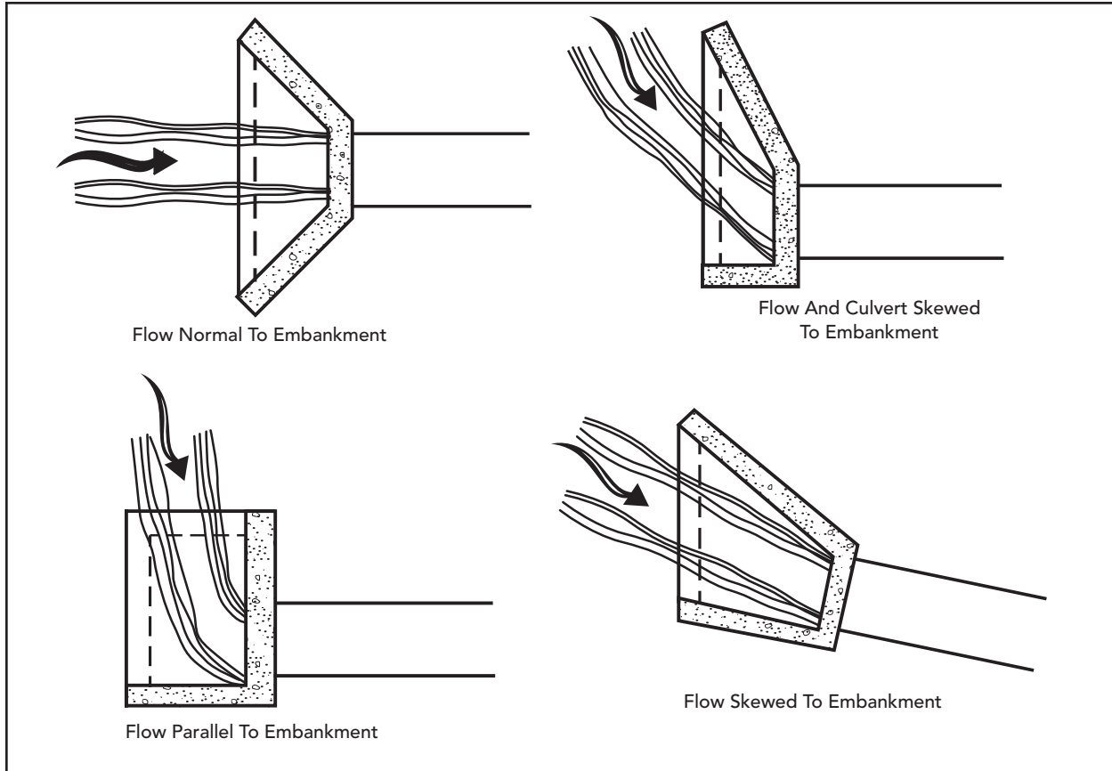
Figure 4-1 Typical Headwall and Wingwall Configurations
