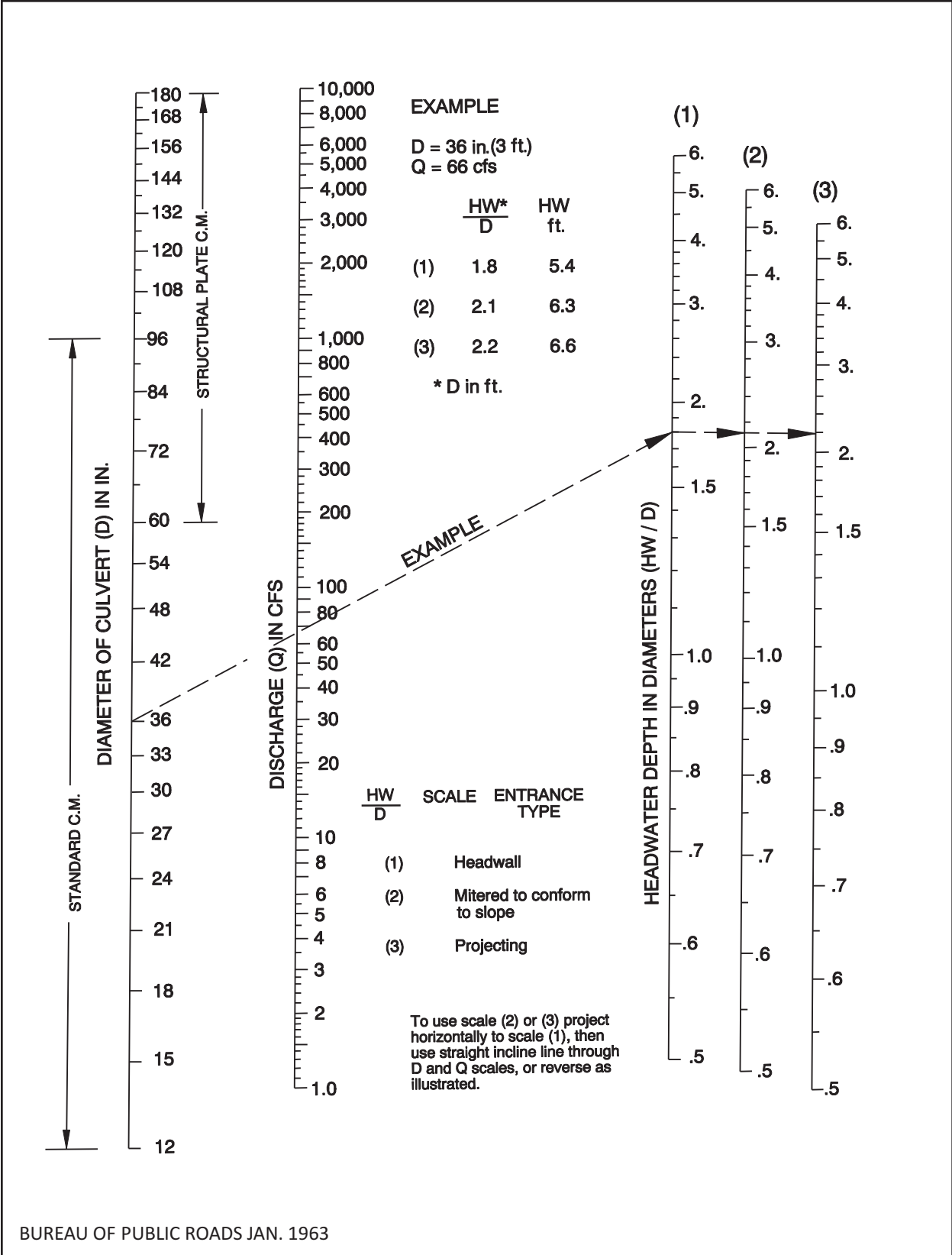
Figure 4-A-5 Headwater Depth For C. M. Pipe Culverts With Inlet Control
