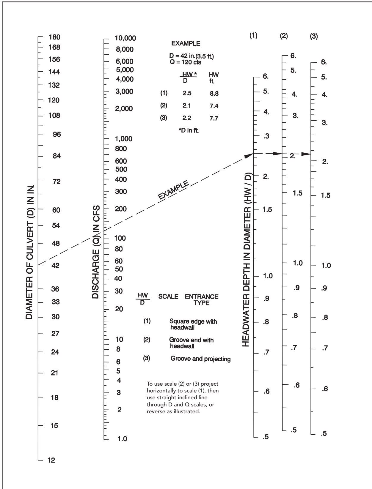
Figure 4-2 Headwater Depth for Concrete Pipe Culverts with Inlet Control
